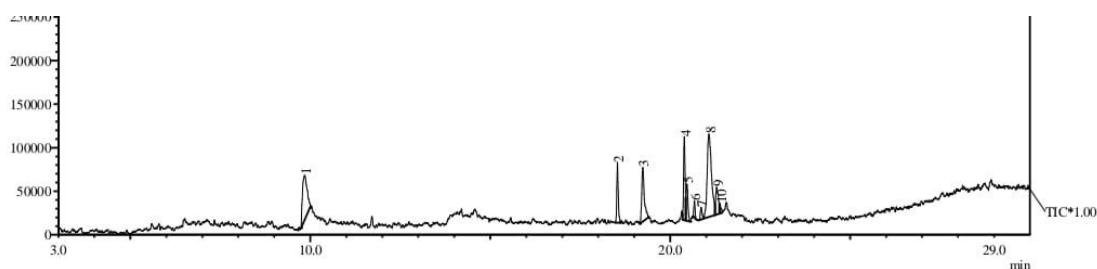
Figure -4 Chromotogram of secondary metabolities of P.griseoroseum before mutation.
